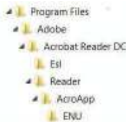
Gambar 3.5 Struktur Folder
